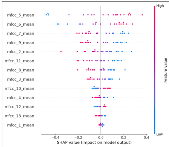
(a) Shap global MFCCs.
